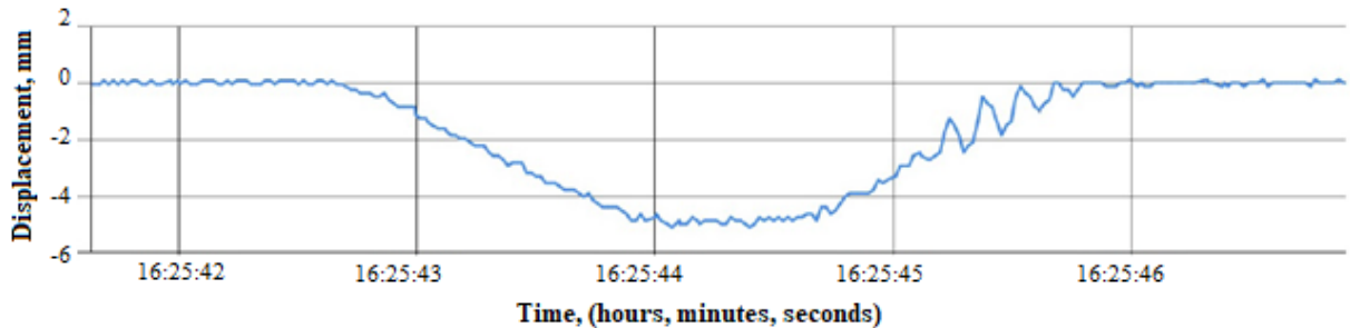
Figure 2. Diagram of deflections (displacements) of the superstructure (23.6 m) during the passage of TEM-18 and freight cars at a speed of 90 km/h [Author's own material]
