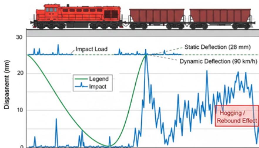
Figure 3. Dynamics of vertical displacements in the middle of a 23.6 m long span (train speed 90 km/h) [Author's own material]
