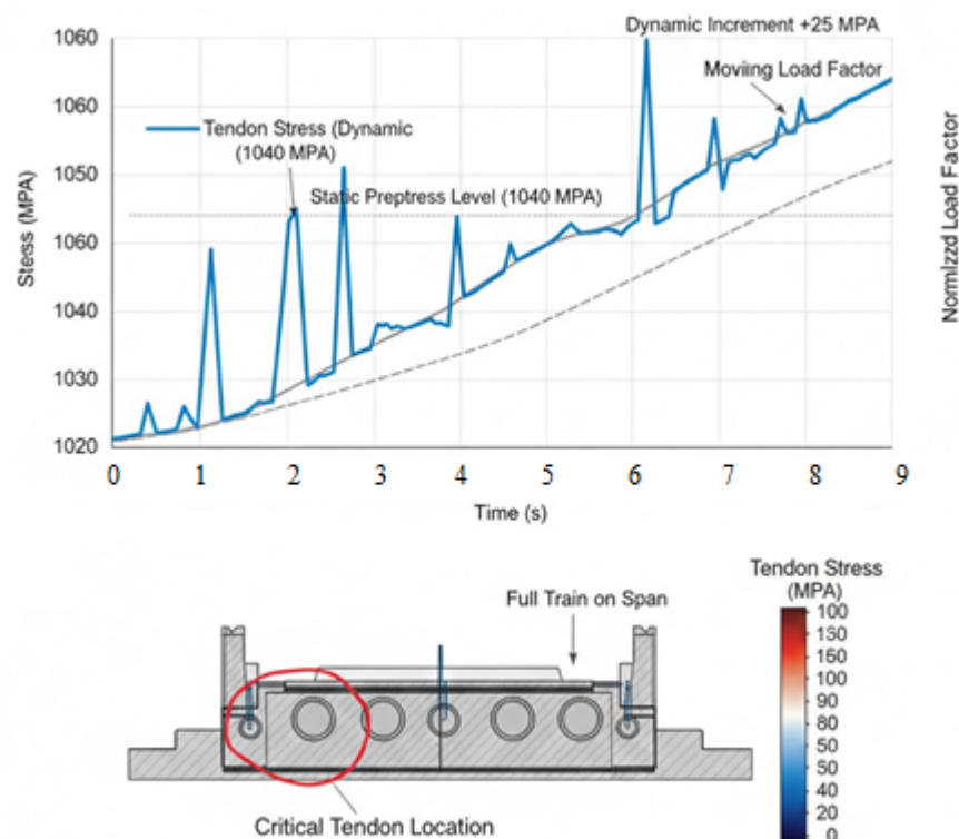
Figure 6. Dynamic stress history within a typical 23.6 m prestressed span, showing static prestress levels exceeded when traveling at 90 km/h [Author's own material]
