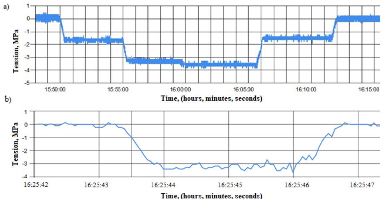
Figure 1. Diagrams of tensile stresses of a middle span of 23.6 m long: a) statics; b) at a speed of 90 km/h. [Author's own material]
